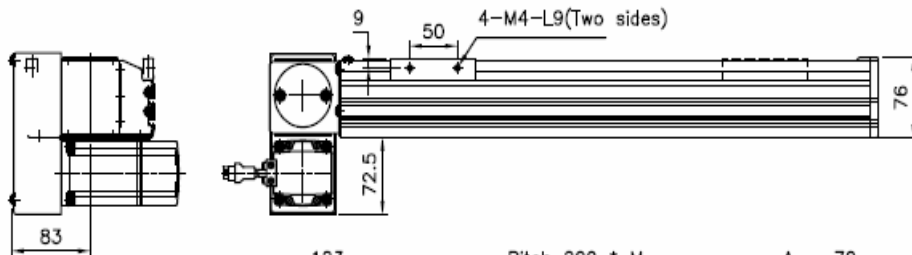
"A" DETAIL CHART
