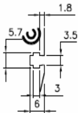
"A" DETAIL CHART
